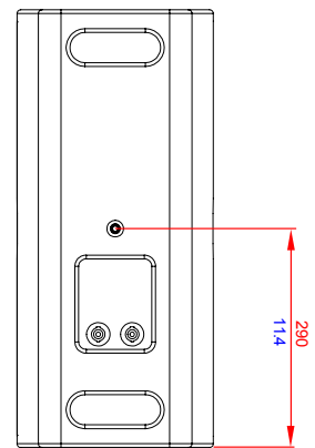
REAR
