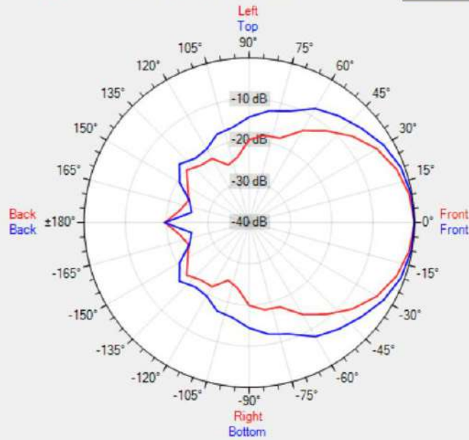
Data Shown: MPLT62 (Apart Audio) Display Parameters: Frequency: 2000Hz (1/24th Octave)
