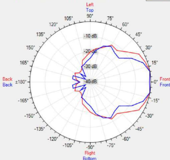
Data Shown: MPLT62 (Apart Audio) Display Parameters: Frequency: 8000Hz (1/24th Octave)
