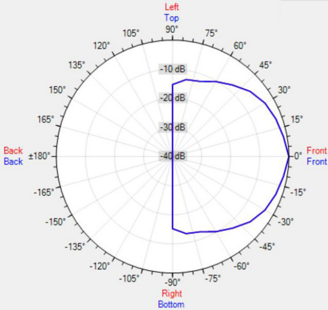
Data Shown: CMAR5 (Apart Audio) Display Parameters: Frequency: 4000Hz (1/24th Octave)
