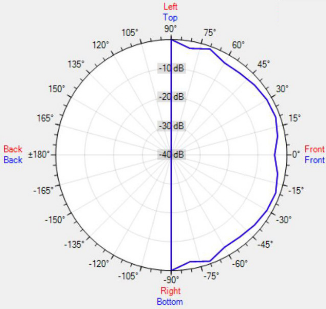
Data Shown: CMAR5 (Apart Audio) Display Parameters: Frequency: 1000Hz (1/24th Octave)
