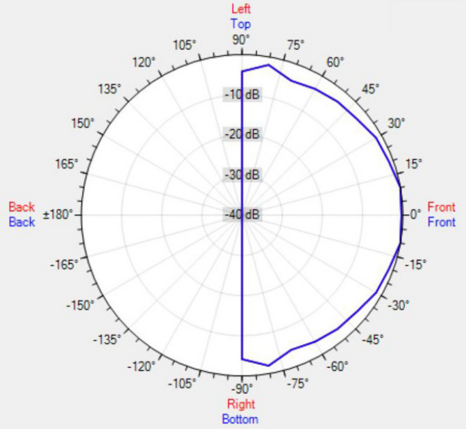
Data Shown: CMAR5 (Apart Audio) Display Parameters: Frequency: 2000Hz (1/24th Octave)
