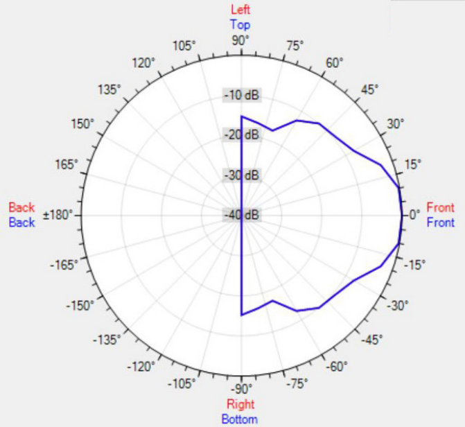
Data Shown: CMAR5 (Apart Audio) Display Parameters: Frequency: 8000Hz (1/24th Octave)
