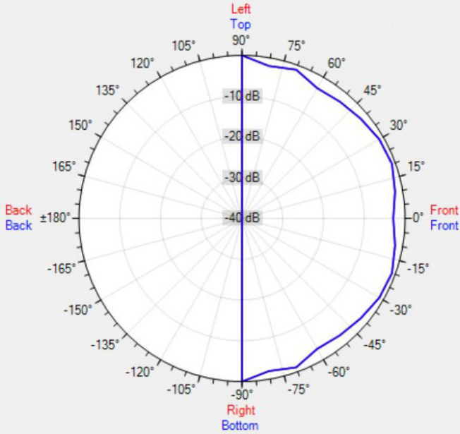
Data Shown: CMAR6 (Apart Audio) Display Parameters: Frequency: 1000Hz (1/24th Octave)
