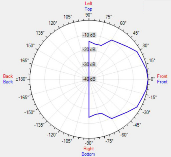
Data Shown: CMAR6 (Apart Audio) Display Parameters: Frequency: 8000Hz (1/24th Octave)
