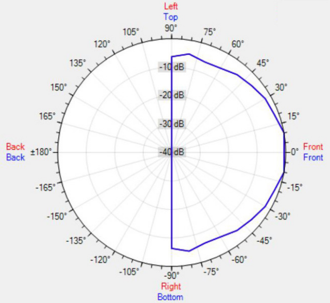
Data Shown: CMAR6 (Apart Audio) Display Parameters: Frequency: 2000Hz (1/24th Octave)
