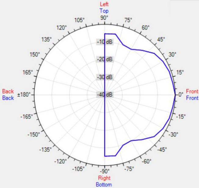
Data Shown: CMAR6 (Apart Audio) Display Parameters: Frequency: 4000Hz (1/24th Octave)
