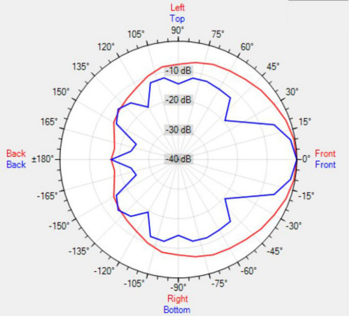
Data Shown: COLS41 (Apart Audio) Display Parameters: Frequency: 2000Hz (1/24th Octave)
