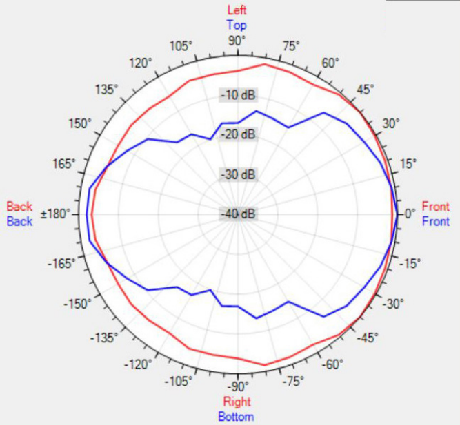
Data Shown: COLS41 (Apart Audio) Display Parameters: Frequency: 1000Hz (1/24th Octave)
