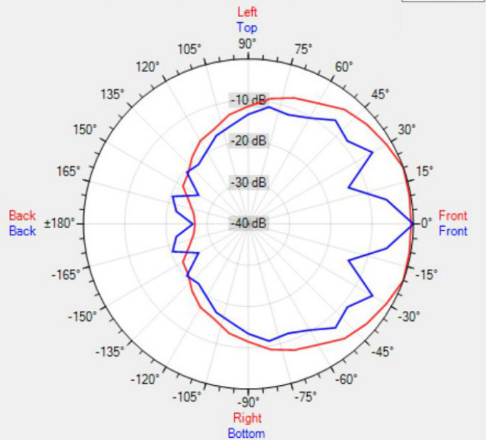
Data Shown: COLS41 (Apart Audio) Display Parameters: Frequency: 8000Hz (1/24th Octave)
