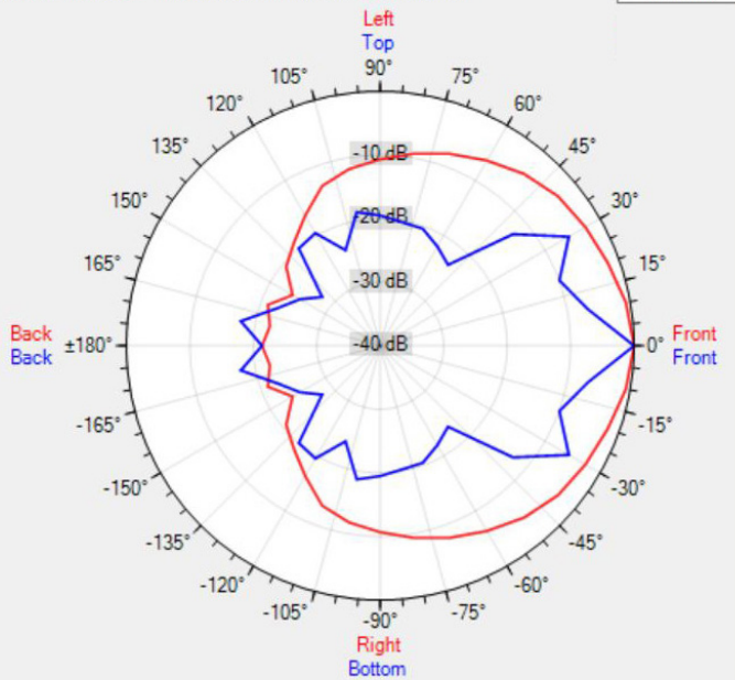
Data Shown: COLS41 (Apart Audio) Display Parameters: Frequency: 4000Hz (1/24th Octave)
