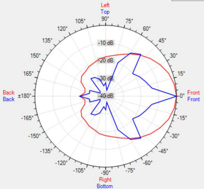
Data Shown: COLW101 (Apart Audio) Display Parameters: Frequency: 4000Hz (1/24th Octave)
