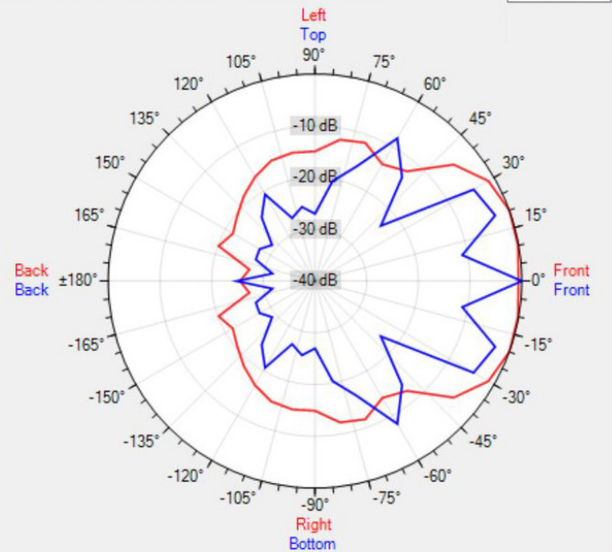
- Please recalculate balloon - Data Shown: COLW81 (Apart Audio) Display Parameters: Frequency: 8000Hz (1/24th Octave)
