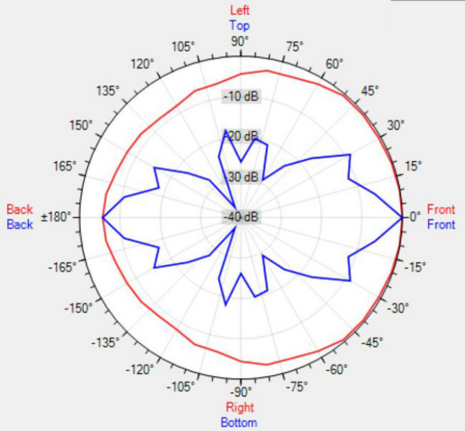
Data Shown: COLW101 (Apart Audio) Display Parameters: Frequency: 1000Hz (1/24th Octave)
