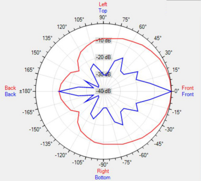
Data Shown: COLW101 (Apart Audio) Display Parameters: Frequency: 2000Hz (1/24th Octave)
