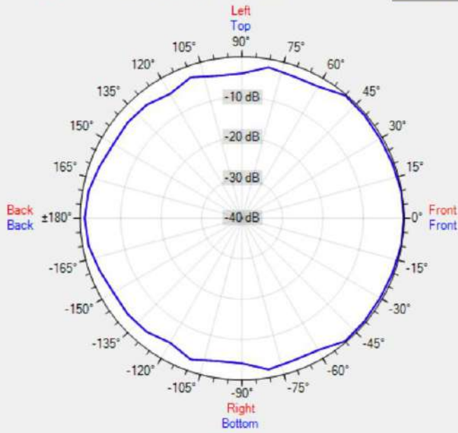
Data Shown: MASK2 (Apart Audio) Display Parameters: Frequency: 1000Hz (1/24th Octave)
