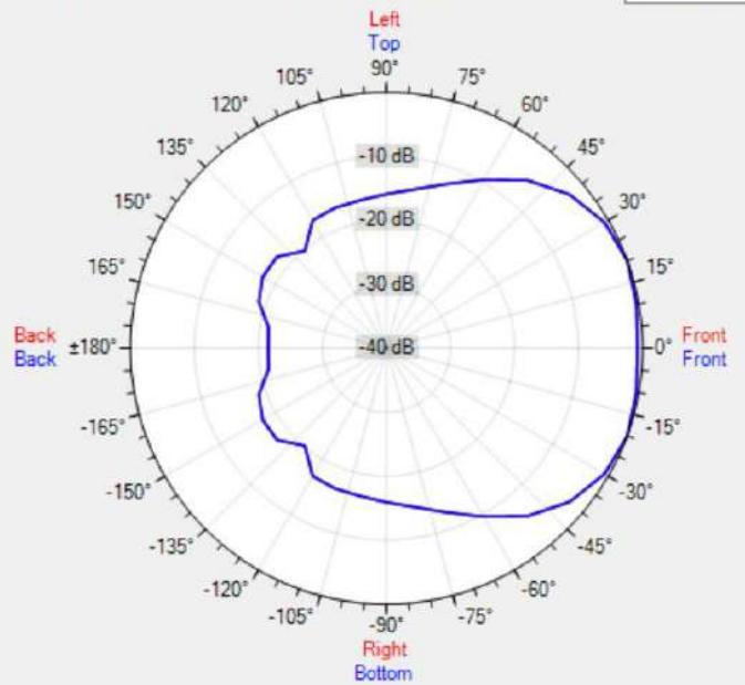
Data Shown: MASK2 (Apart Audio) Display Parameters: Frequency: 8000Hz (1/24th Octave)
