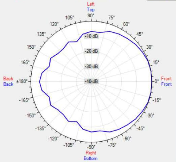
Data Shown: MASK2 (Apart Audio) Display Parameters: Frequency: 2000Hz (1/24th Octave)
