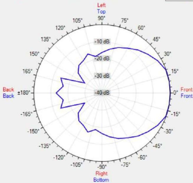
Data Shown: MASK2 (Apart Audio) Display Parameters: Frequency: 4000Hz (1/24th Octave)
