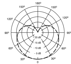
典型指向性图样
