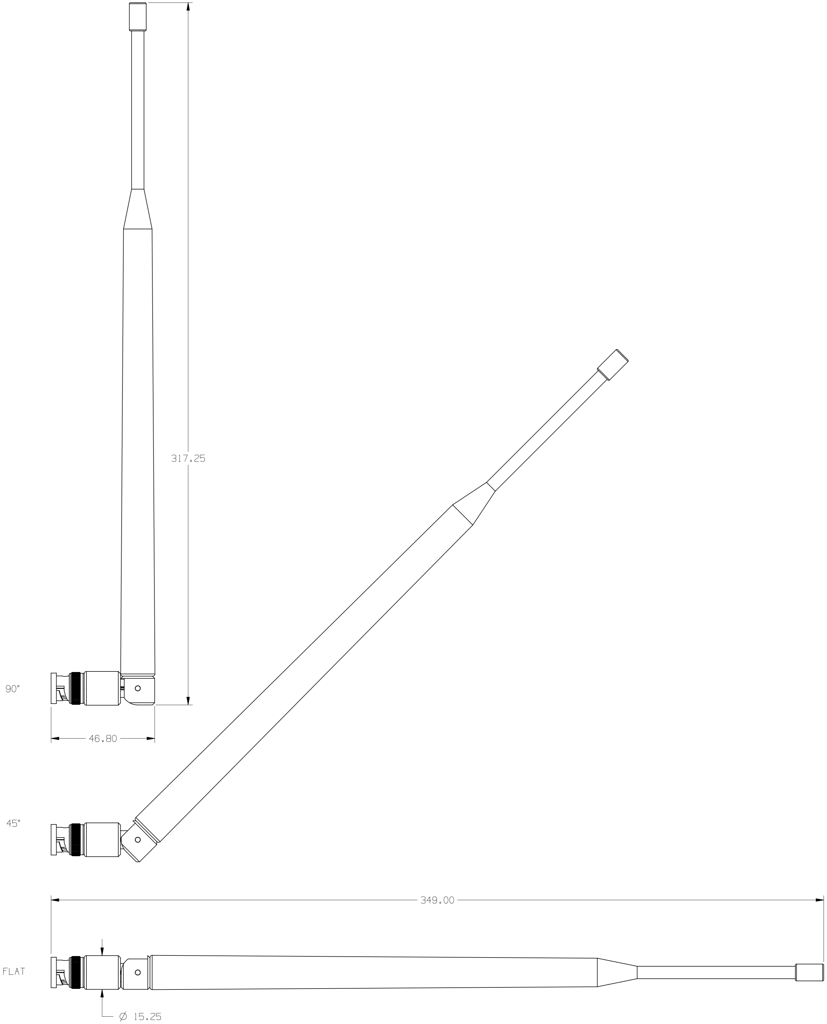
SHURE UA8-470-636 - HALF WAVE ANTENNA SCALE 1:1 ALL DIMENSIONS SHOWN IN mm ASSEMBLY LENGTH MAY VARY DEPENDENT ON OPERATING FREQUENCY
