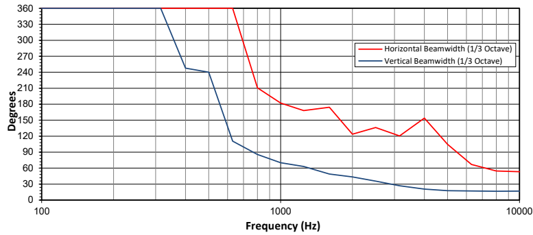
Beamwidth vs Frequency (@ 5m/16.4ft)
