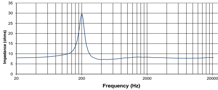
Impedance vs frequency
