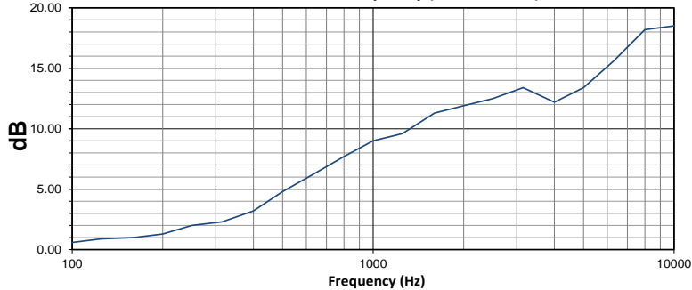
DI vs Frequency (@ 5m/16.4ft)
