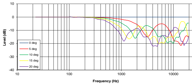
Upper Vertical Off-axis Frequency Response, Normalized On-Axis
