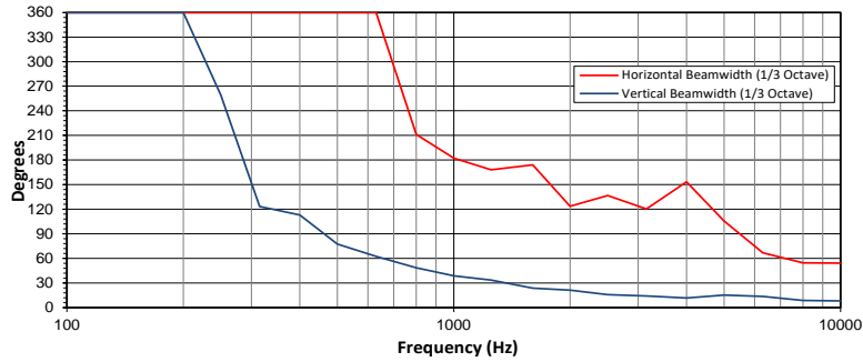
Beamwidth vs Frequency (@ 5m/16.4ft)
