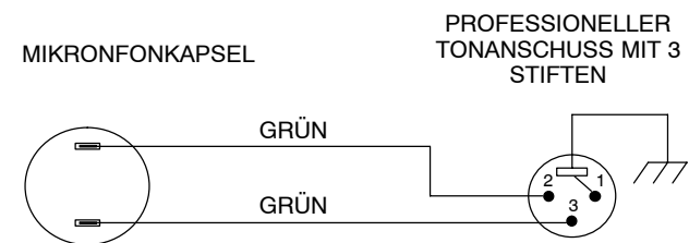
INTERNE ANSCHLÜSSE
