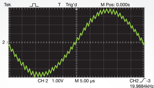
In a conventional Class D amplifier the switching ripple is present on the output audio waveform as a superimposed high frequency ripple. The result is a distorted signal and EMI emissions on output cabling.
